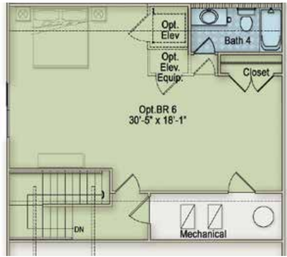
OPTIONAL BEDROOM THIRD FLOOR
