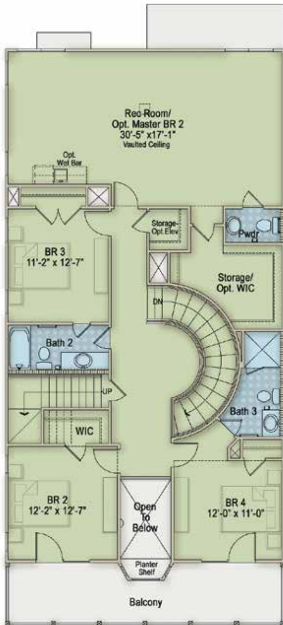
SECOND FLOOR WITH THIRD FLOOR OPTION
