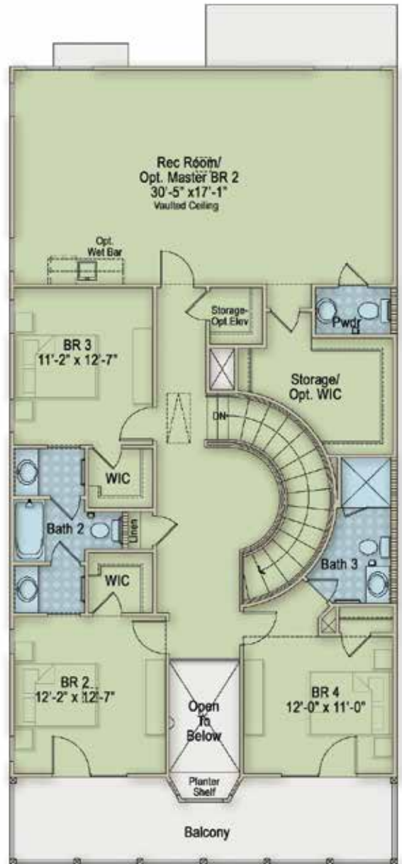
SECOND FLOOR WITH NO THIRD FLOOR
